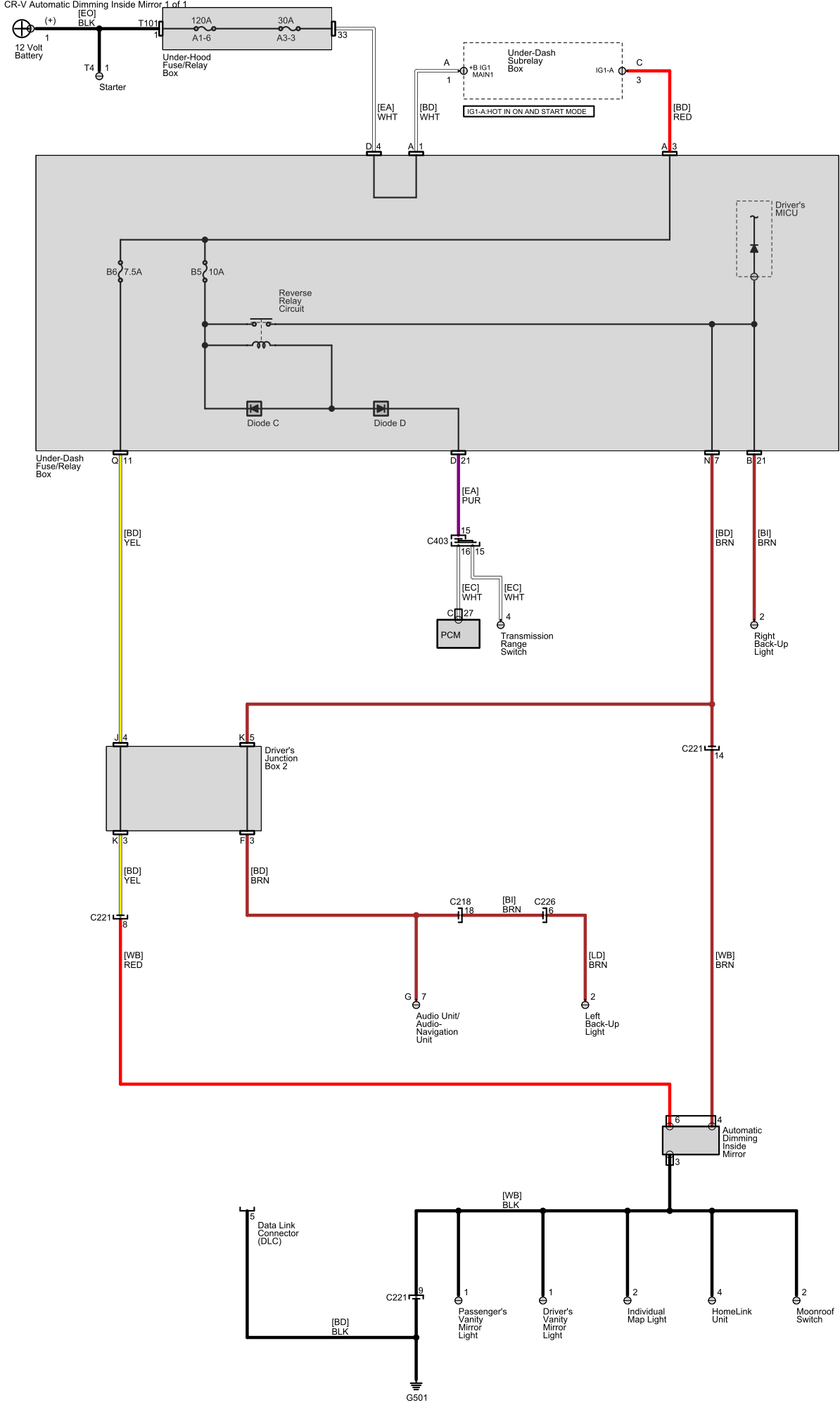
CR-V Automatic Dimming Inside Mirror 1 of 1
